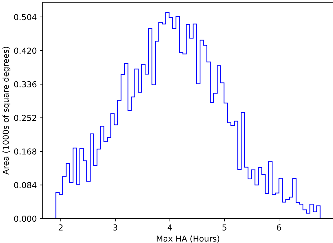
too_elab_heavy_r64_d3_ugrizy_v3.4_10yrs WFD u band: Max HA
