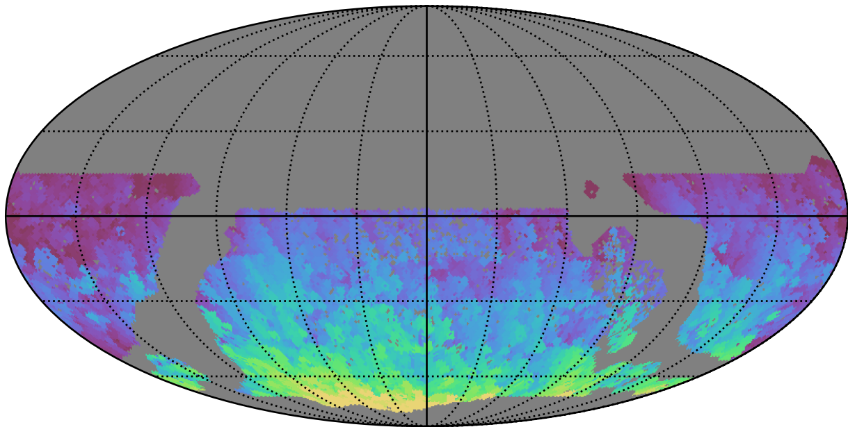
too_elab_heavy_r64_d3_ugrizy_v3.4_10yrs WFD r band: Max HA
