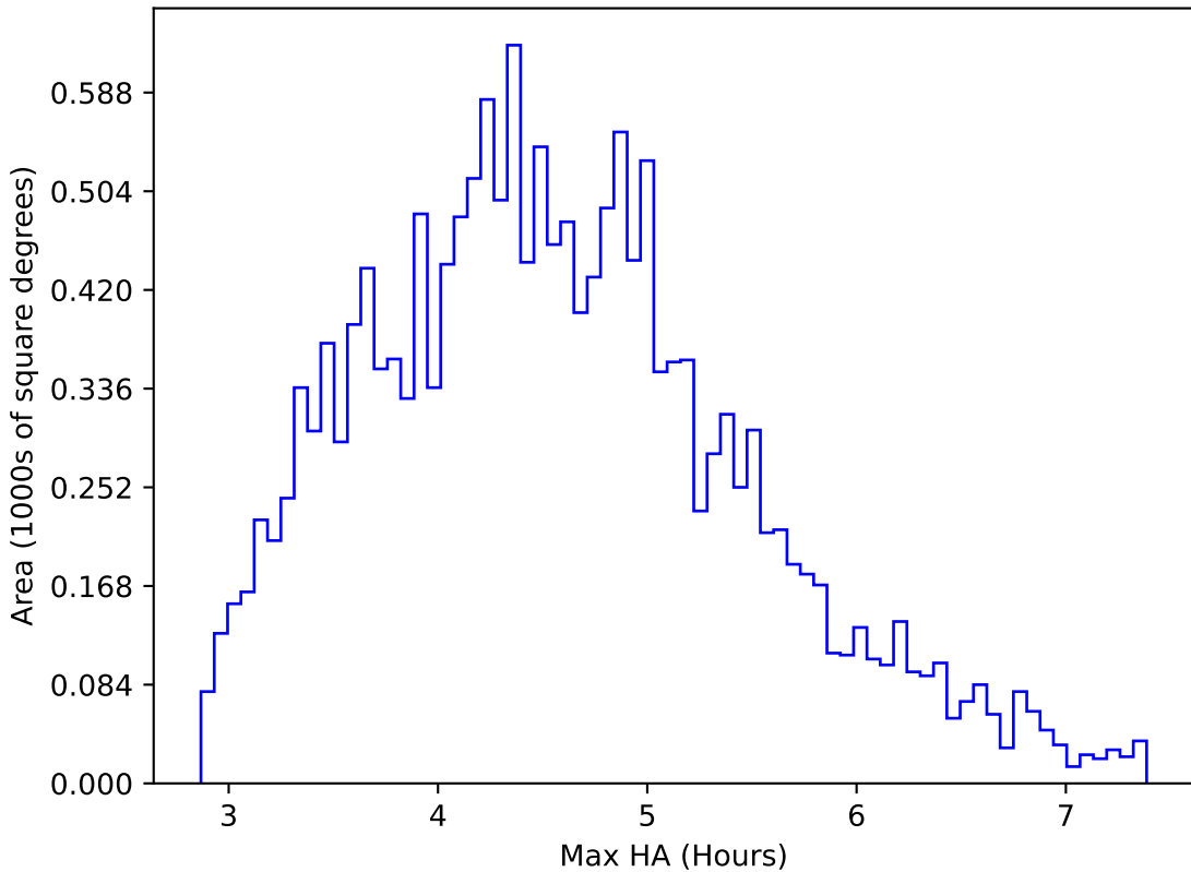
too_elab_heavy_r64_d3_ugrizy_v3.4_10yrs WFD r band: Max HA
