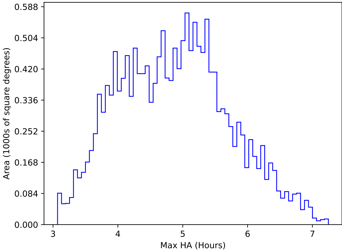
too_elab_heavy_r64_d3_ugrizy_v3.4_10yrs WFD i band: Max HA
