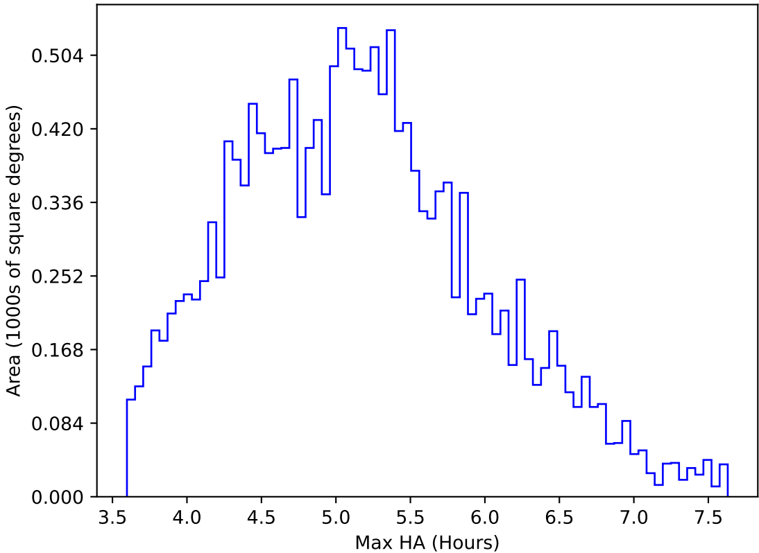
too_elab_heavy_r64_d3_ugrizy_v3.4_10yrs WFD all bands: Max HA
