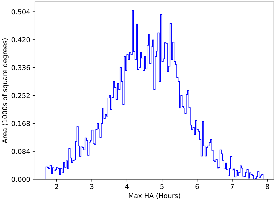
too_elab_heavy_r64_d3_ugrizy_v3.4_10yrs All sky z band: Max HA
