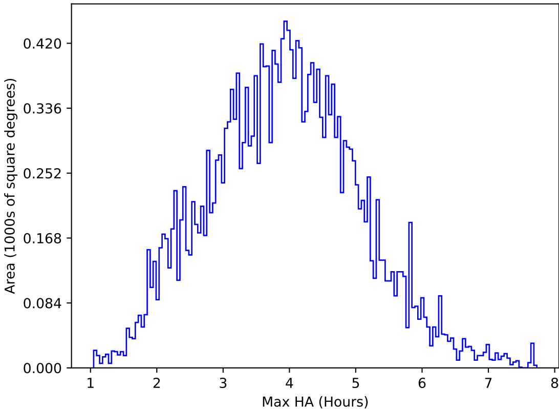
too_elab_heavy_r64_d3_ugrizy_v3.4_10yrs All sky u band: Max HA
