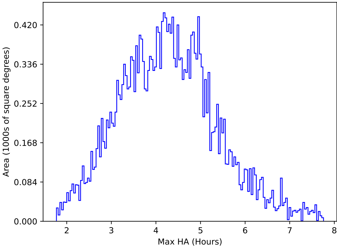
too_elab_heavy_r64_d3_ugrizy_v3.4_10yrs All sky r band: Max HA
