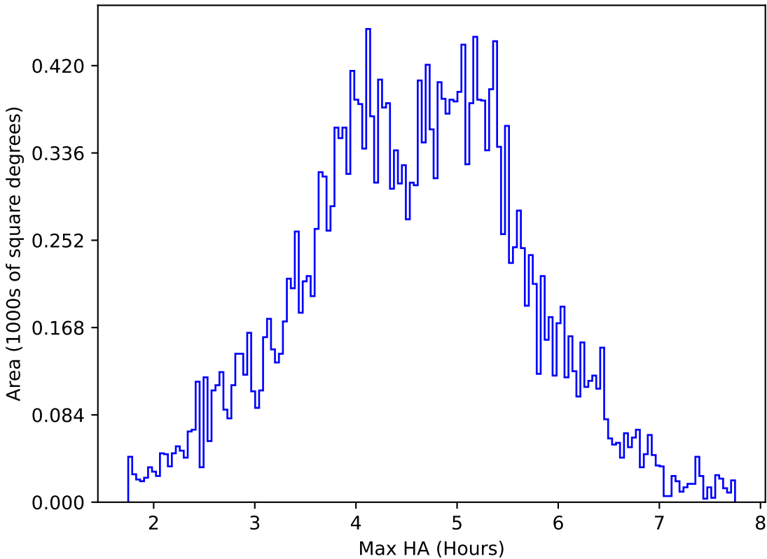
too_elab_heavy_r64_d3_ugrizy_v3.4_10yrs All sky i band: Max HA
