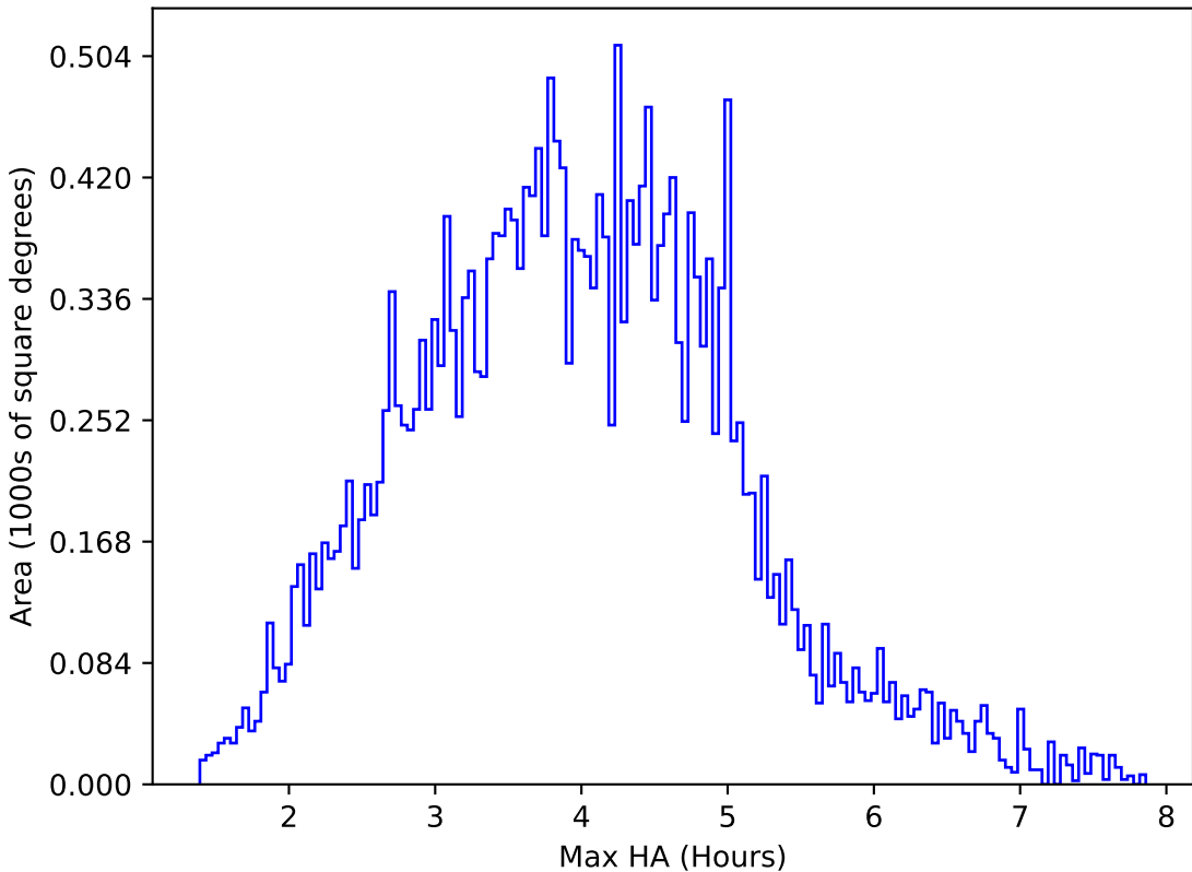
too_elab_heavy_r64_d3_ugrizy_v3.4_10yrs All sky g band: Max HA
