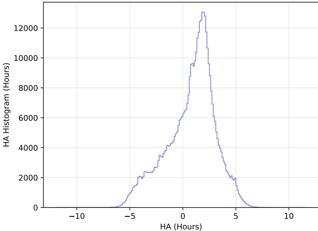
too_elab_heavy_r64_d3_ugrizy_v3.4_10yrs WFD z band: HA Histogram
