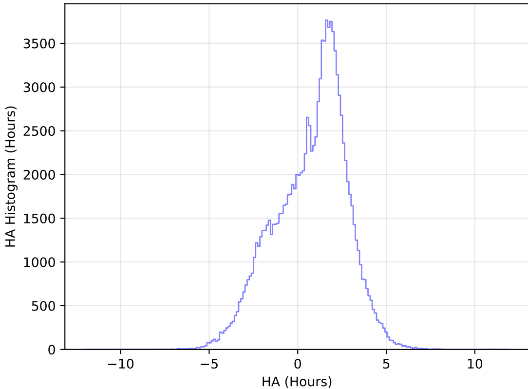
too_elab_heavy_r64_d3_ugrizy_v3.4_10yrs WFD u band: HA Histogram
