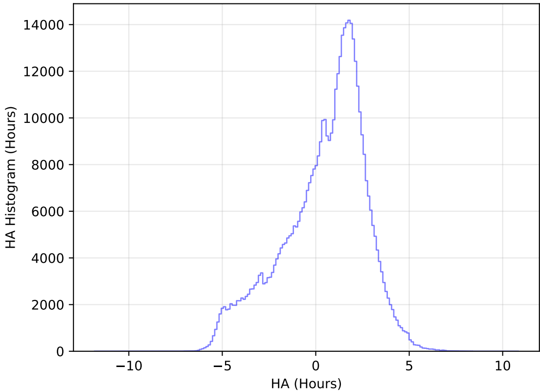
too_elab_heavy_r64_d3_ugrizy_v3.4_10yrs WFD r band: HA Histogram
