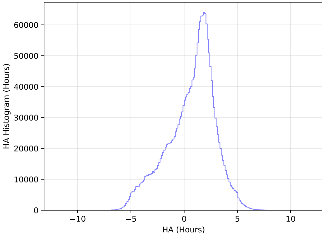
too_elab_heavy_r64_d3_ugrizy_v3.4_10yrs WFD all bands: HA Histogram
