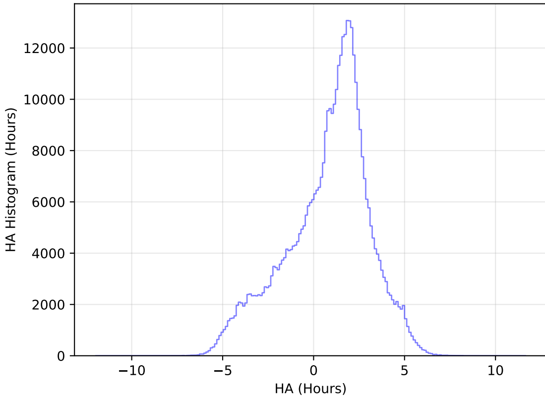
too_elab_heavy_r64_d3_ugrizy_v3.4_10yrs All sky z band: HA Histogram
