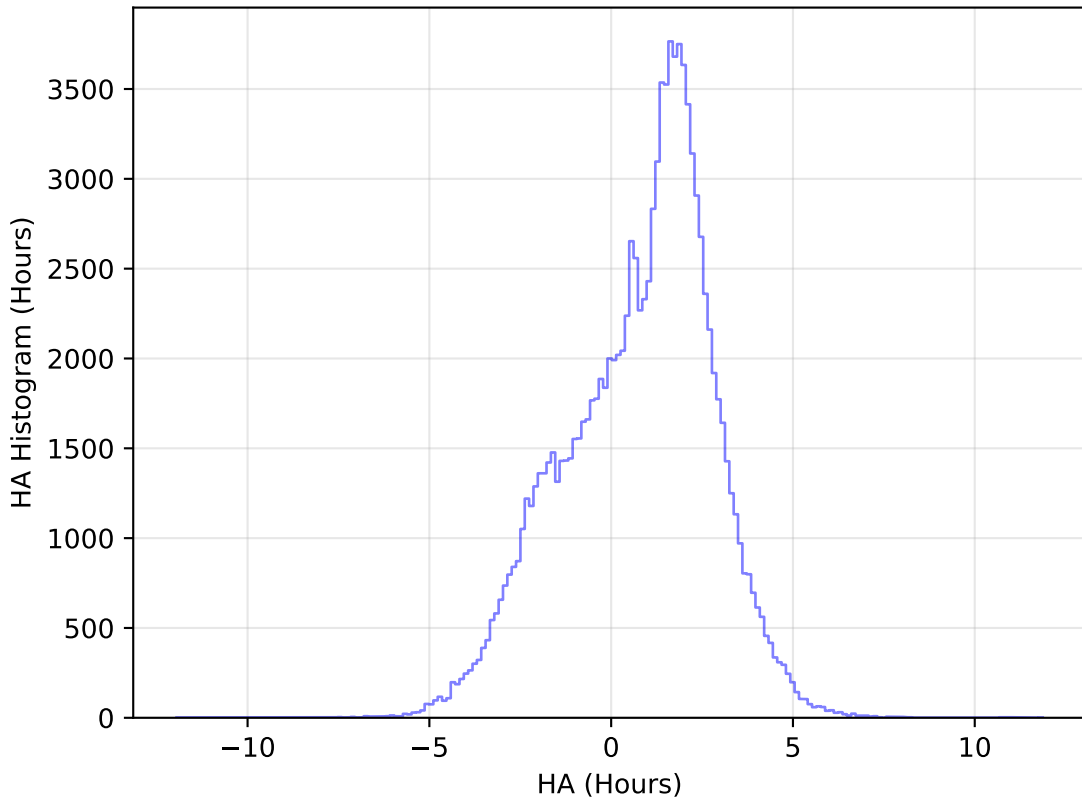
too_elab_heavy_r64_d3_ugrizy_v3.4_10yrs All sky u band: HA Histogram
