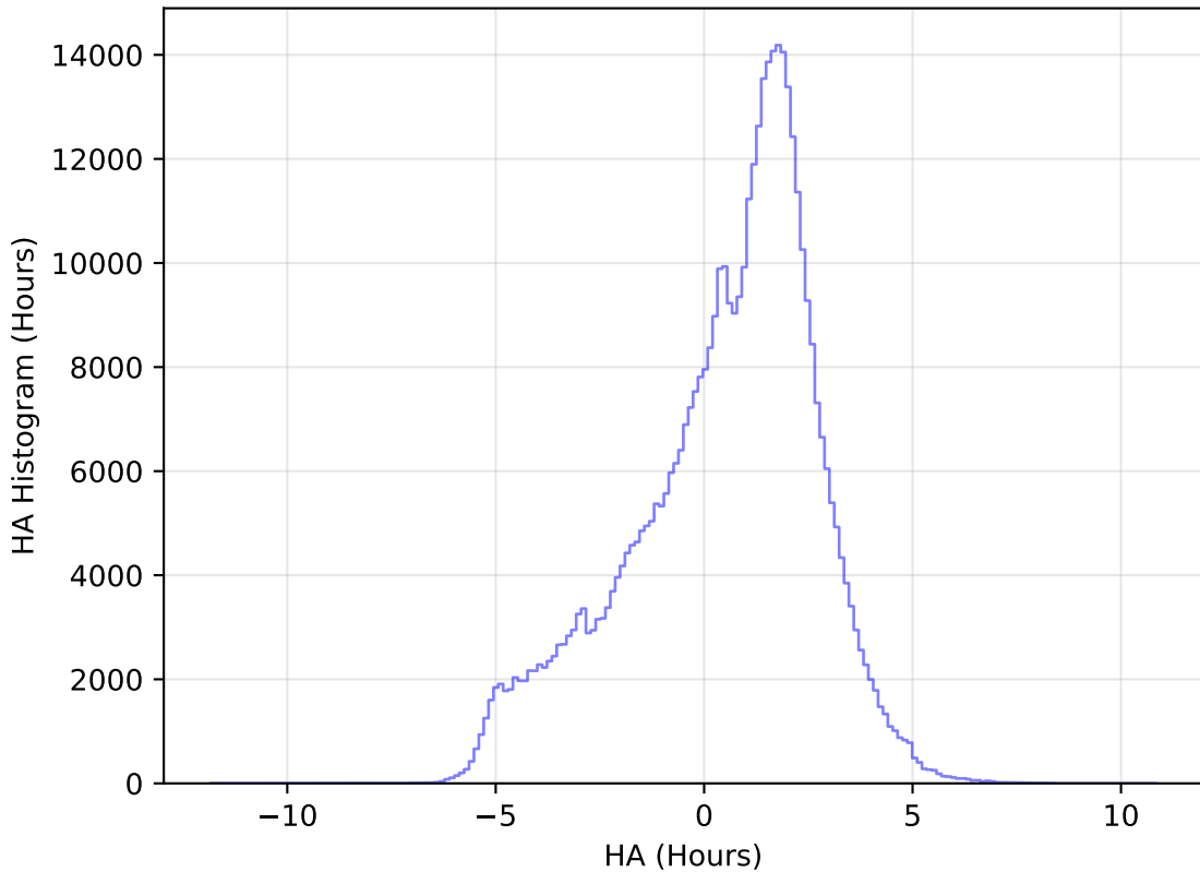
too_elab_heavy_r64_d3_ugrizy_v3.4_10yrs All sky r band: HA Histogram
