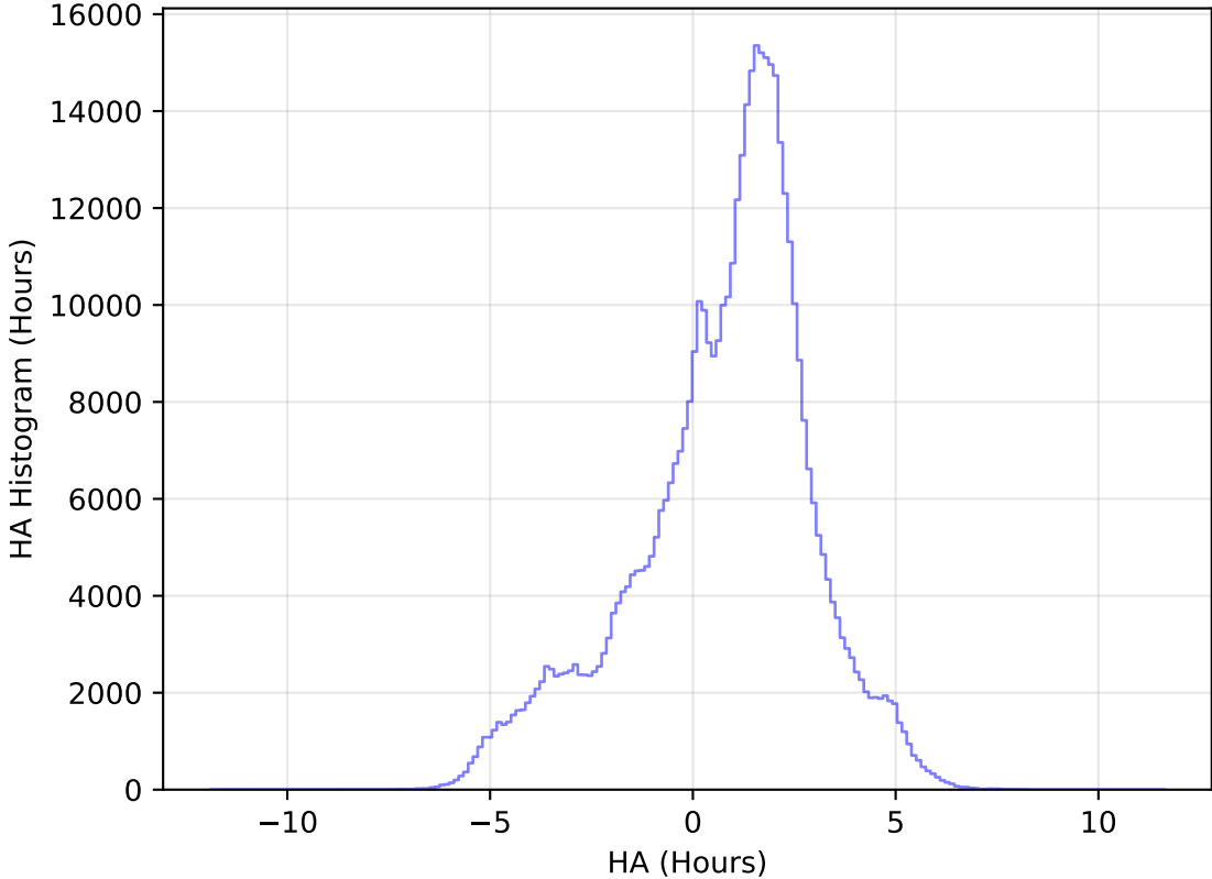
too_elab_heavy_r64_d3_ugrizy_v3.4_10yrs All sky i band: HA Histogram
