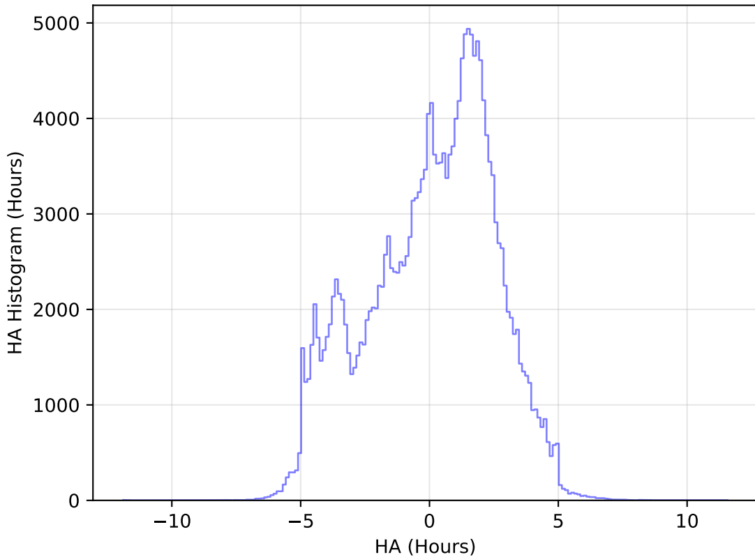
too_elab_heavy_r64_d3_ugrizy_v3.4_10yrs All sky g band: HA Histogram
