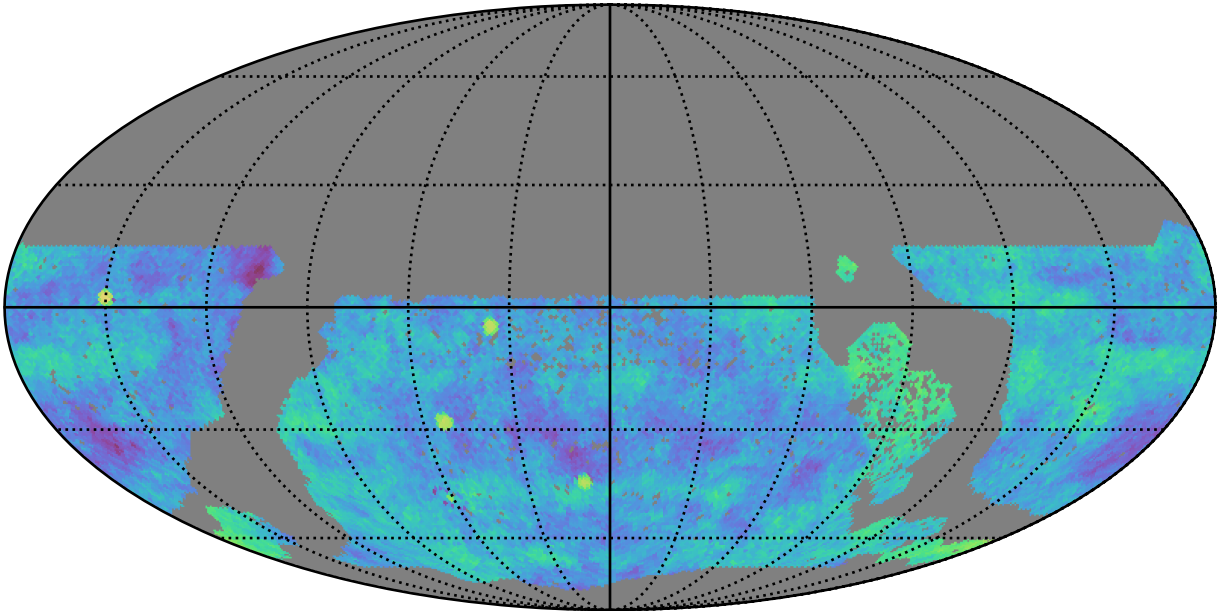
too_elab_heavy_r64_d3_ugrizy_v3.4_10yrs gri WFD: Fraction of visits in pairs (20-90 min)
