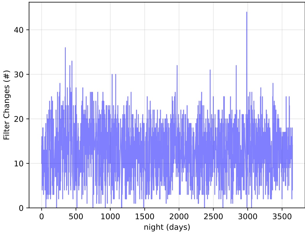
too_elab_heavy_r64_d3_ugrizy_v3.4_10yrs Per Night: Filter Changes
