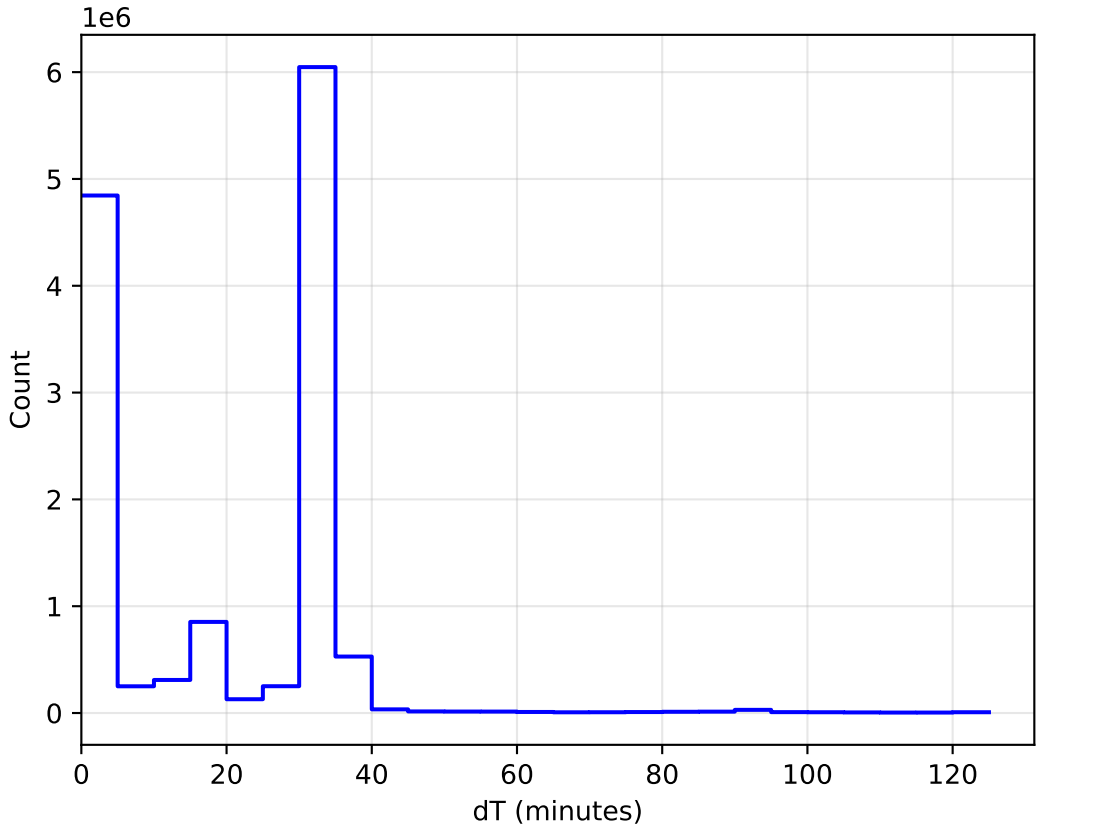
too_elab_heavy_r64_d3_ugrizy_v3.4_10yrs All sky: DeltaT Histogram
