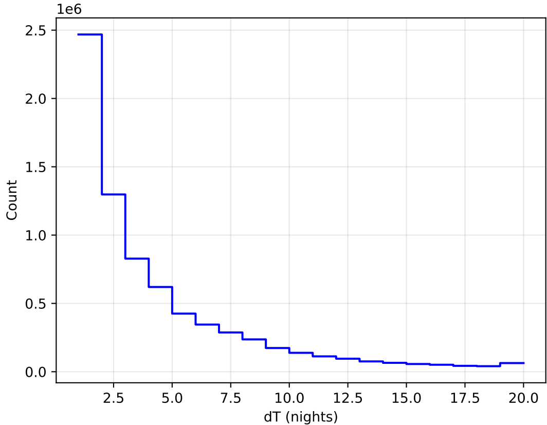
too_elab_heavy_r64_d3_ugrizy_v3.4_10yrs WFD all bands: DeltaNight Histogram
