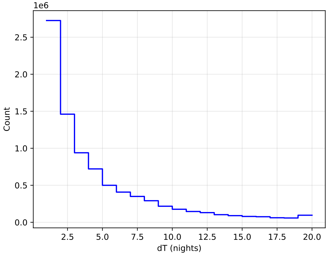
too_elab_heavy_r64_d3_ugrizy_v3.4_10yrs All sky all bands: DeltaNight Histogram
