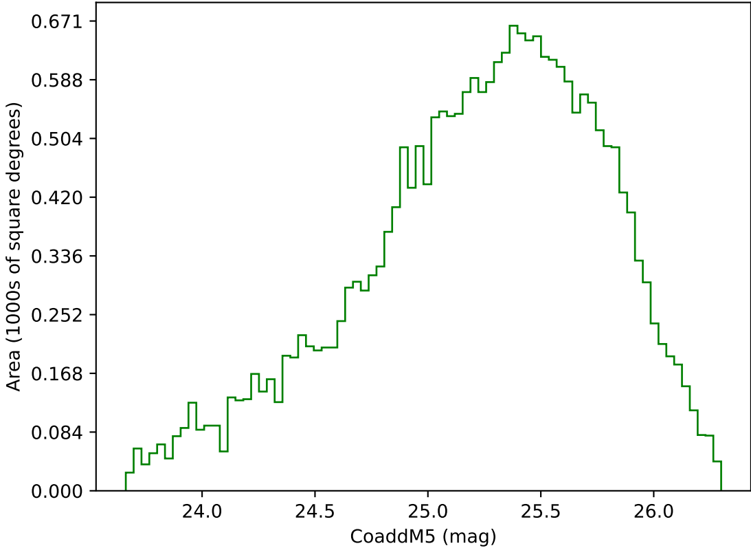
too_elab_heavy_r64_d3_ugrizy_v3.4_10yrs Yr 3-4 g band: CoaddM5
