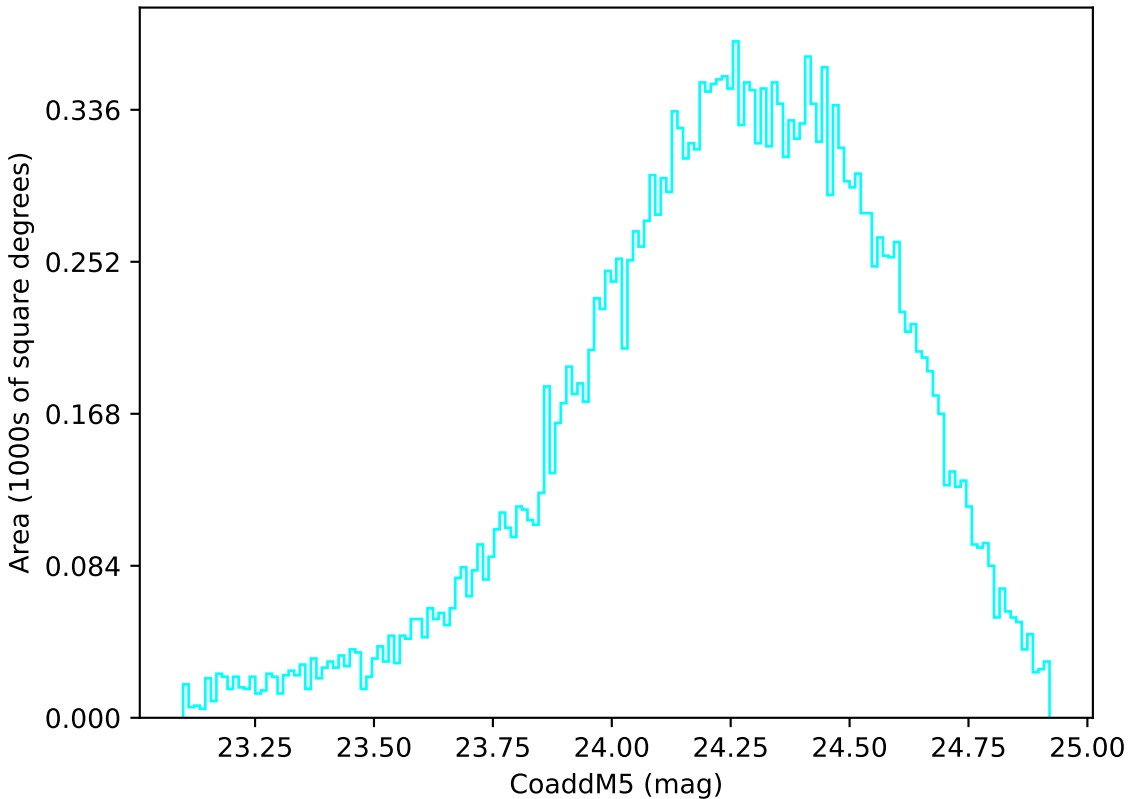
too_elab_heavy_r64_d3_ugrizy_v3.4_10yrs Yr 1 u band: CoaddM5
