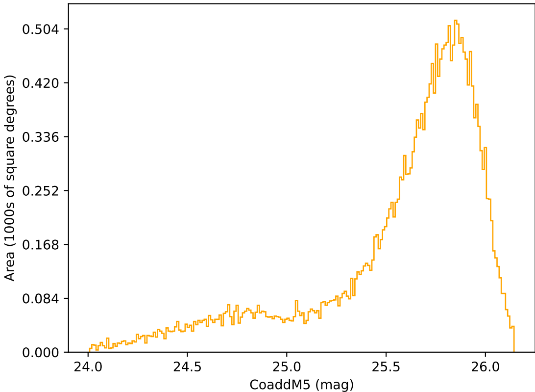
too_elab_heavy_r64_d3_ugrizy_v3.4_10yrs Yr 1 r band: CoaddM5
