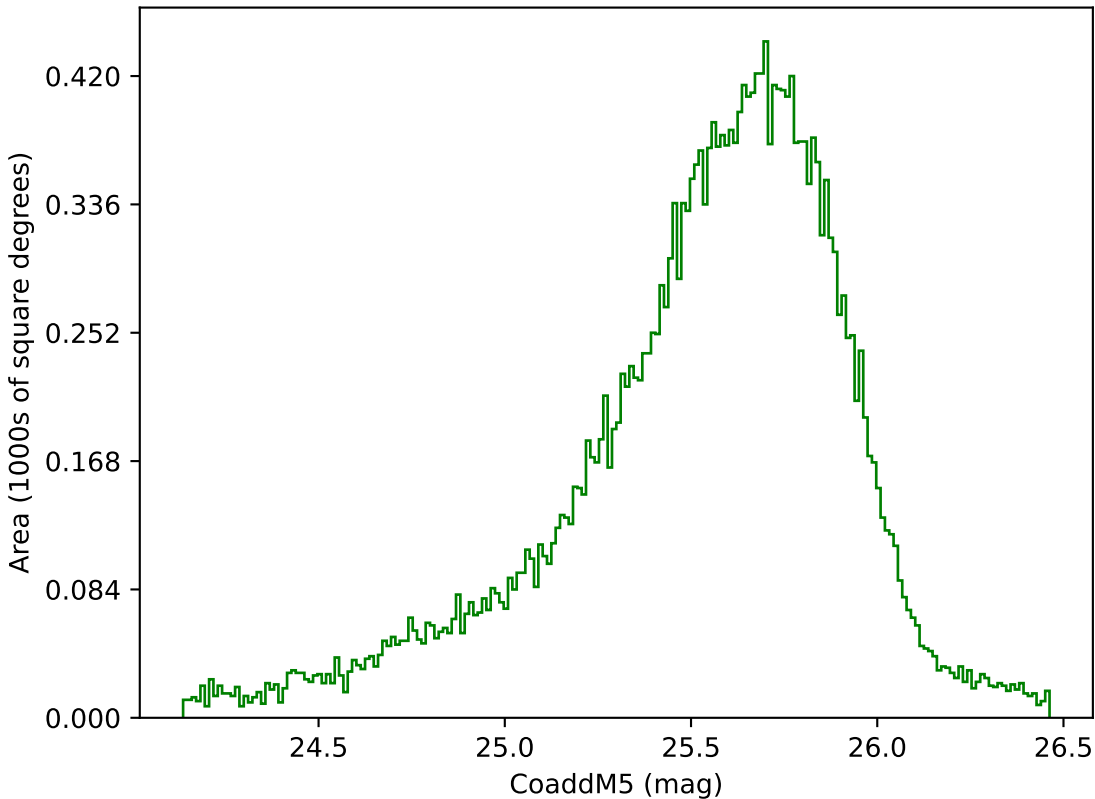
too_elab_heavy_r64_d3_ugrizy_v3.4_10yrs Yr 1 g band: CoaddM5
