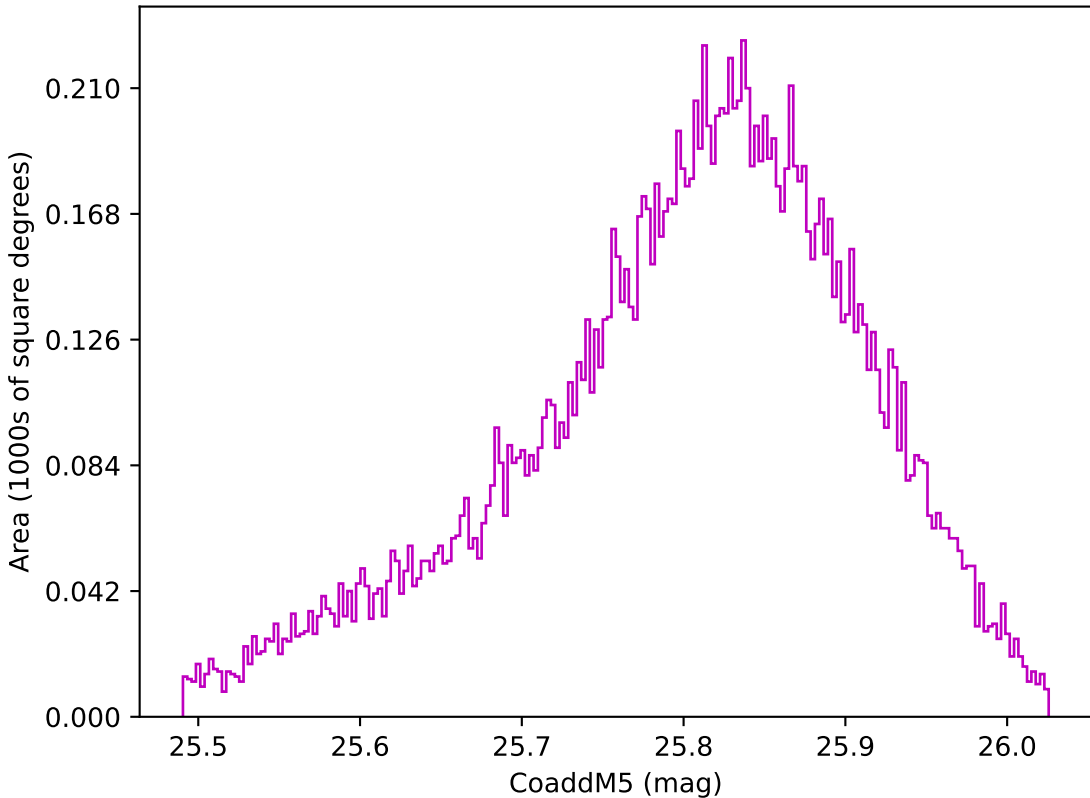
too_elab_heavy_r64_d3_ugrizy_v3.4_10yrs WFD z band: CoaddM5
