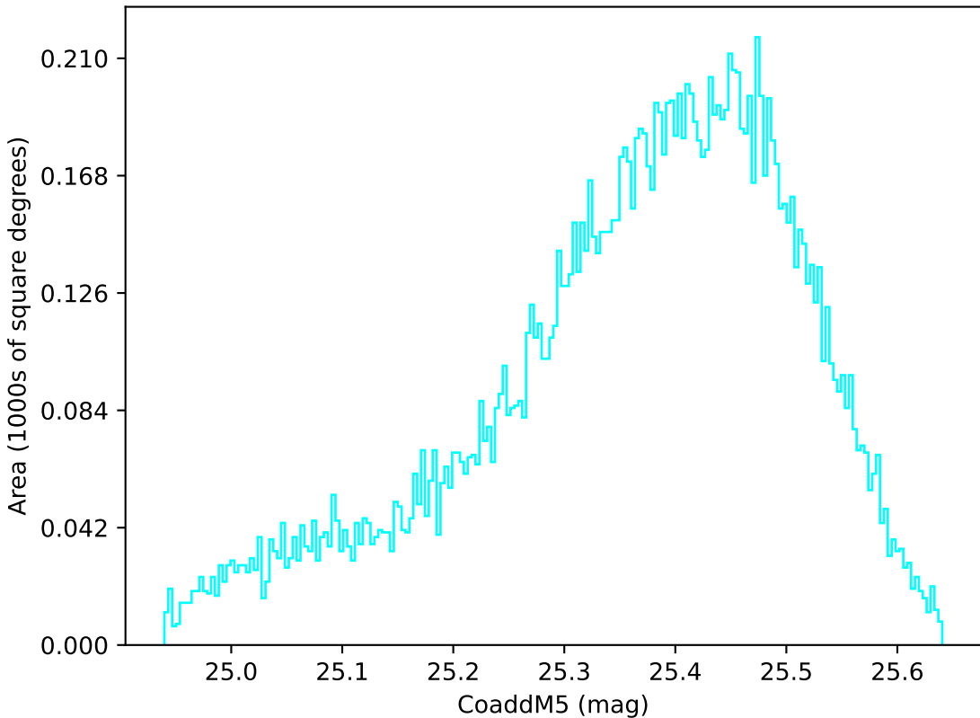
too_elab_heavy_r64_d3_ugrizy_v3.4_10yrs WFD u band: CoaddM5
