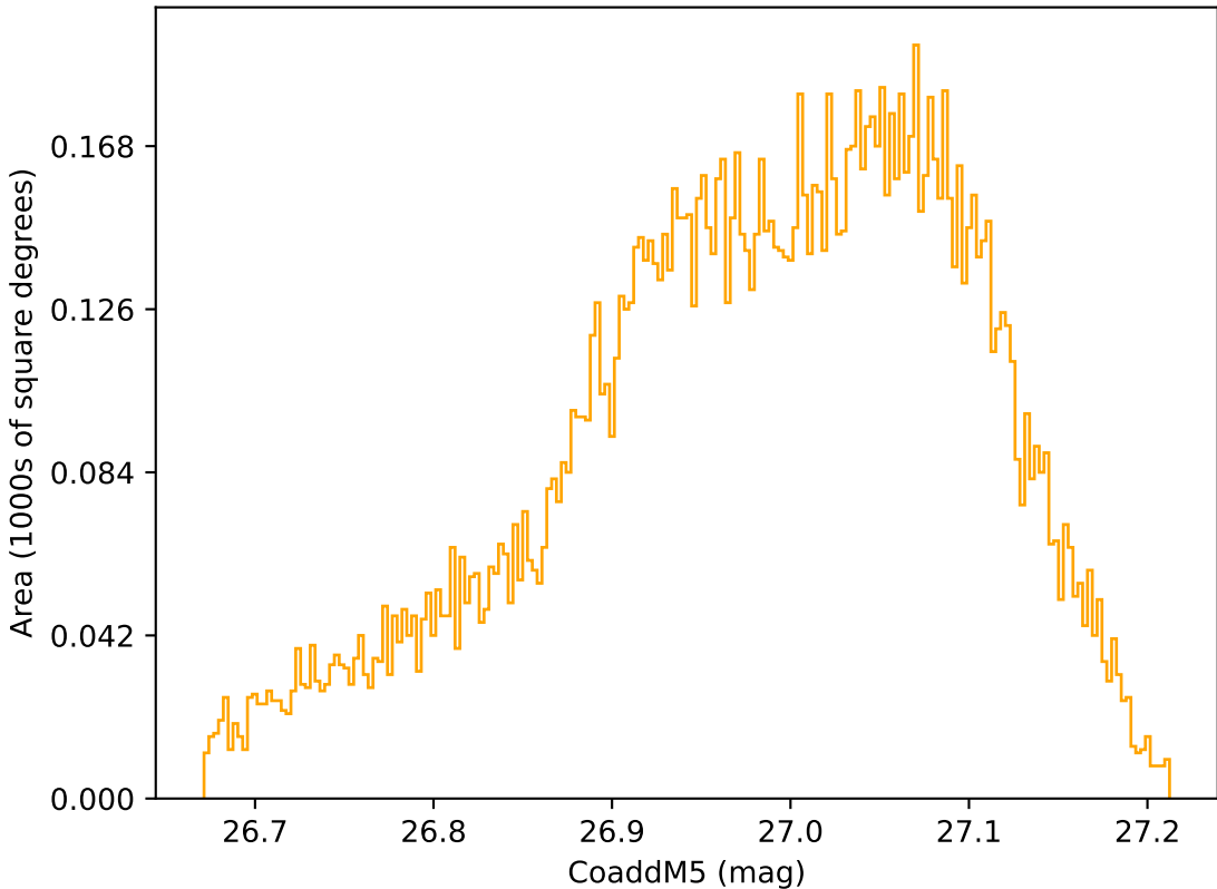
too_elab_heavy_r64_d3_ugrizy_v3.4_10yrs WFD r band: CoaddM5
