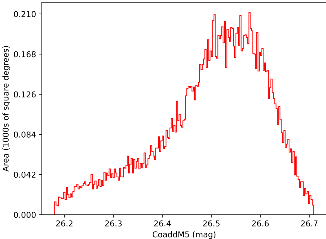
too_elab_heavy_r64_d3_ugrizy_v3.4_10yrs WFD i band: CoaddM5
