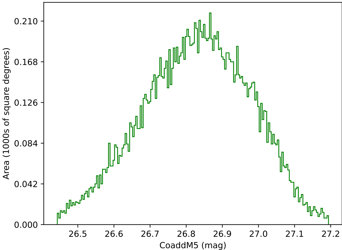
too_elab_heavy_r64_d3_ugrizy_v3.4_10yrs WFD g band: CoaddM5
