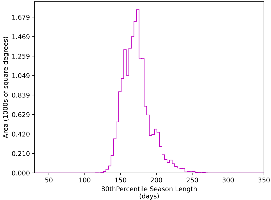
too_elab_heavy_r64_d3_ugrizy_v3.4_10yrs WFD z band: 80thPercentile Season Length
