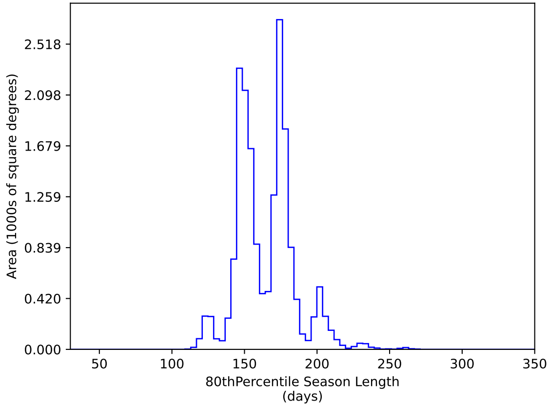
too_elab_heavy_r64_d3_ugrizy_v3.4_10yrs WFD y band: 80thPercentile Season Length
