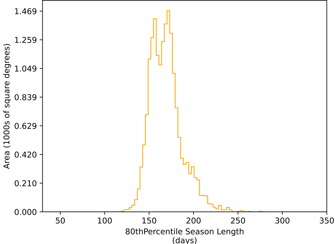
too_elab_heavy_r64_d3_ugrizy_v3.4_10yrs WFD r band: 80thPercentile Season Length
