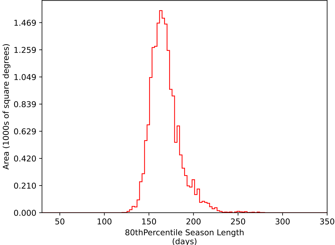
too_elab_heavy_r64_d3_ugrizy_v3.4_10yrs WFD i band: 80thPercentile Season Length
