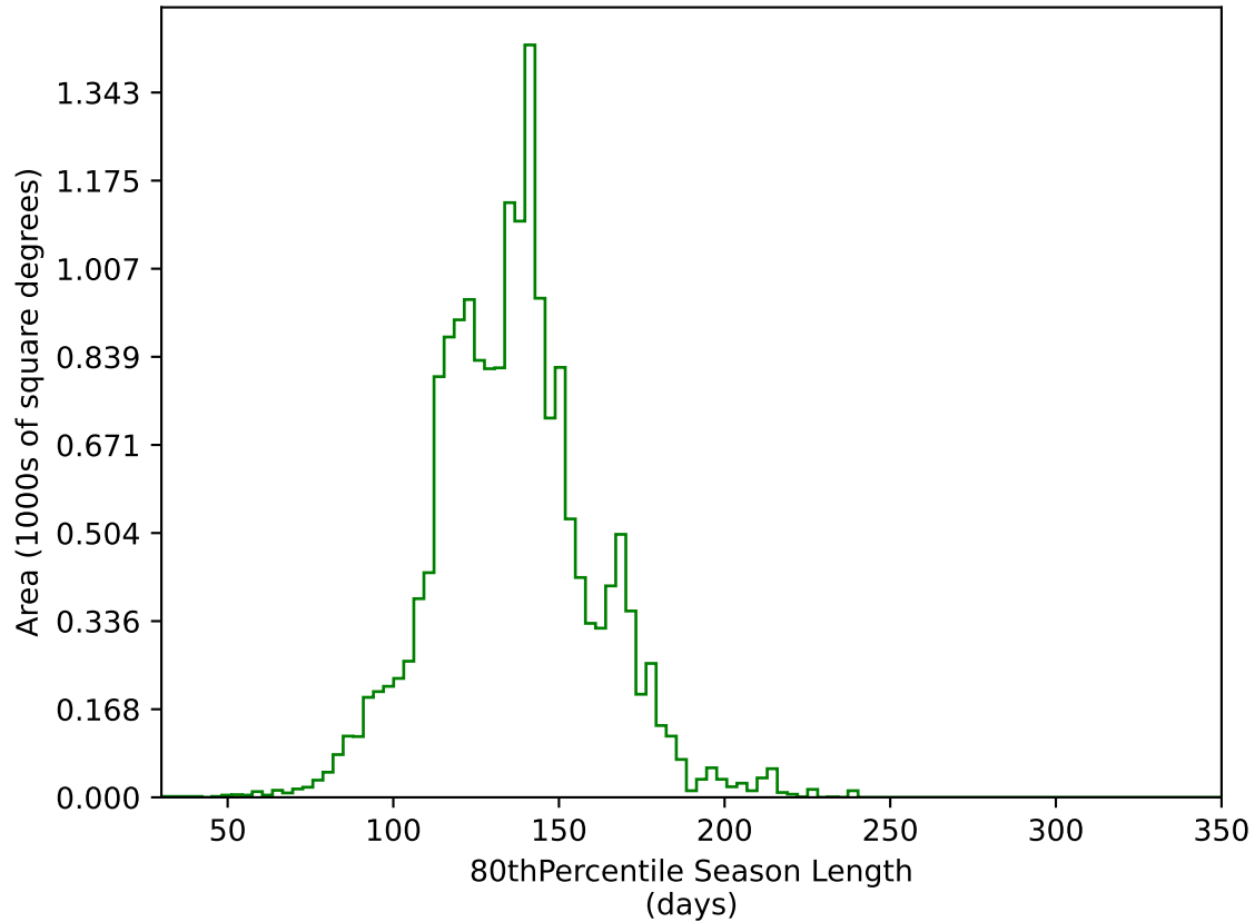
too_elab_heavy_r64_d3_ugrizy_v3.4_10yrs WFD g band: 80thPercentile Season Length
