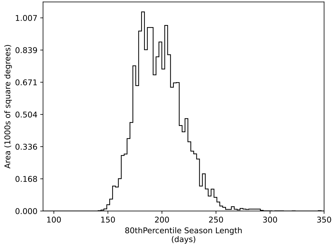
too_elab_heavy_r64_d3_ugrizy_v3.4_10yrs WFD all bands: 80thPercentile Season Length
