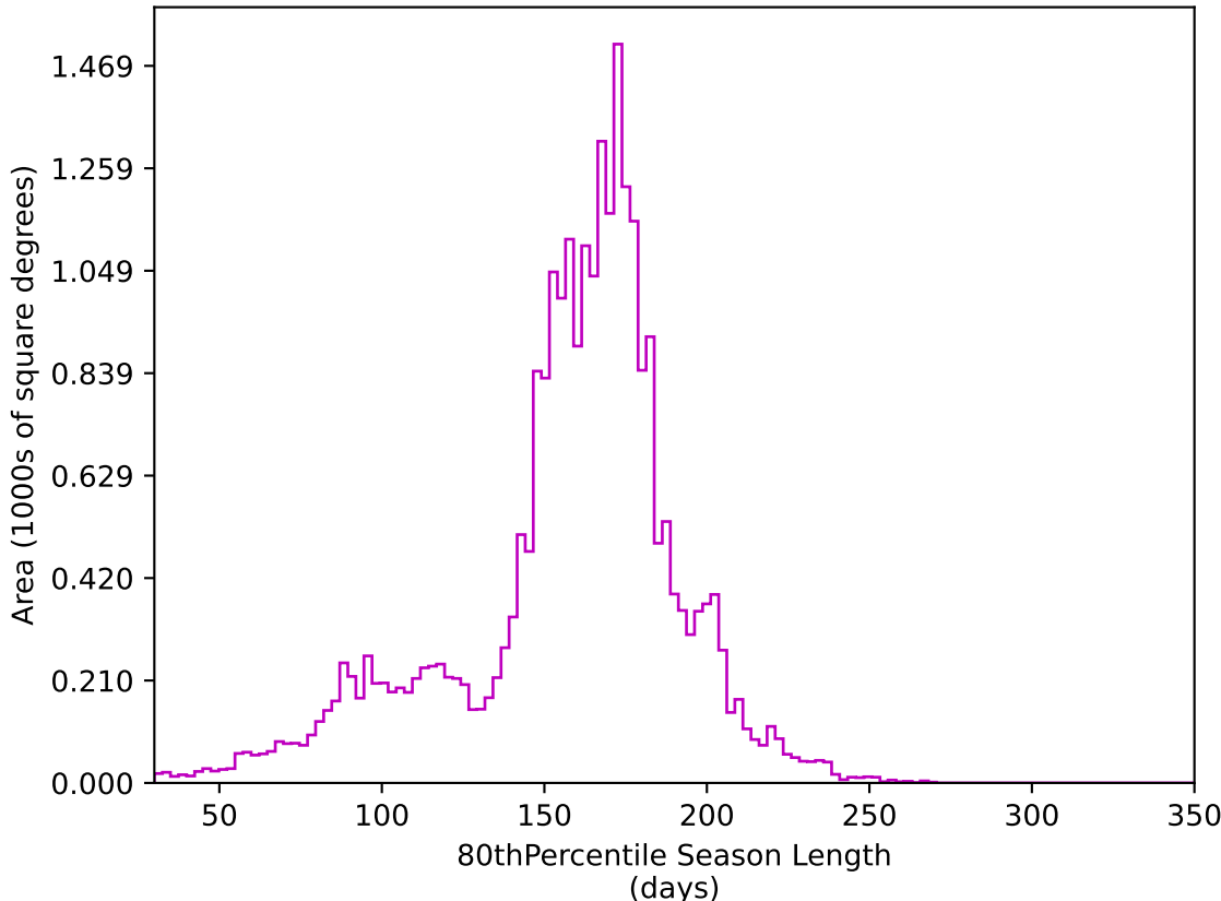
too_elab_heavy_r64_d3_ugrizy_v3.4_10yrs All sky z band: 80thPercentile Season Length
