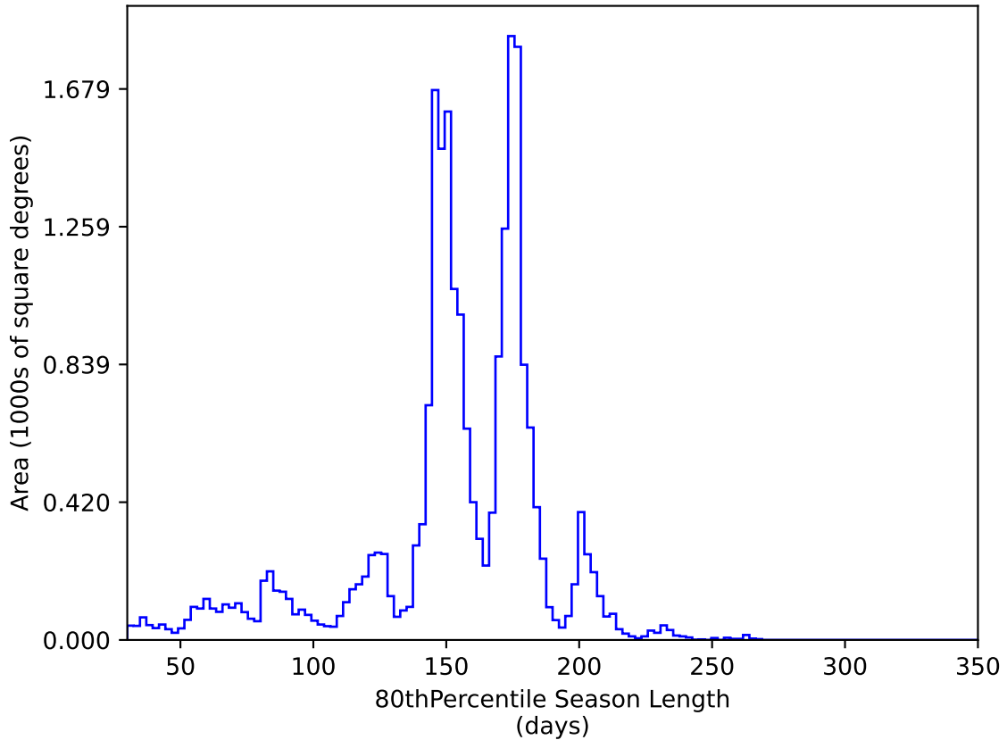
too_elab_heavy_r64_d3_ugrizy_v3.4_10yrs All sky y band: 80thPercentile Season Length
