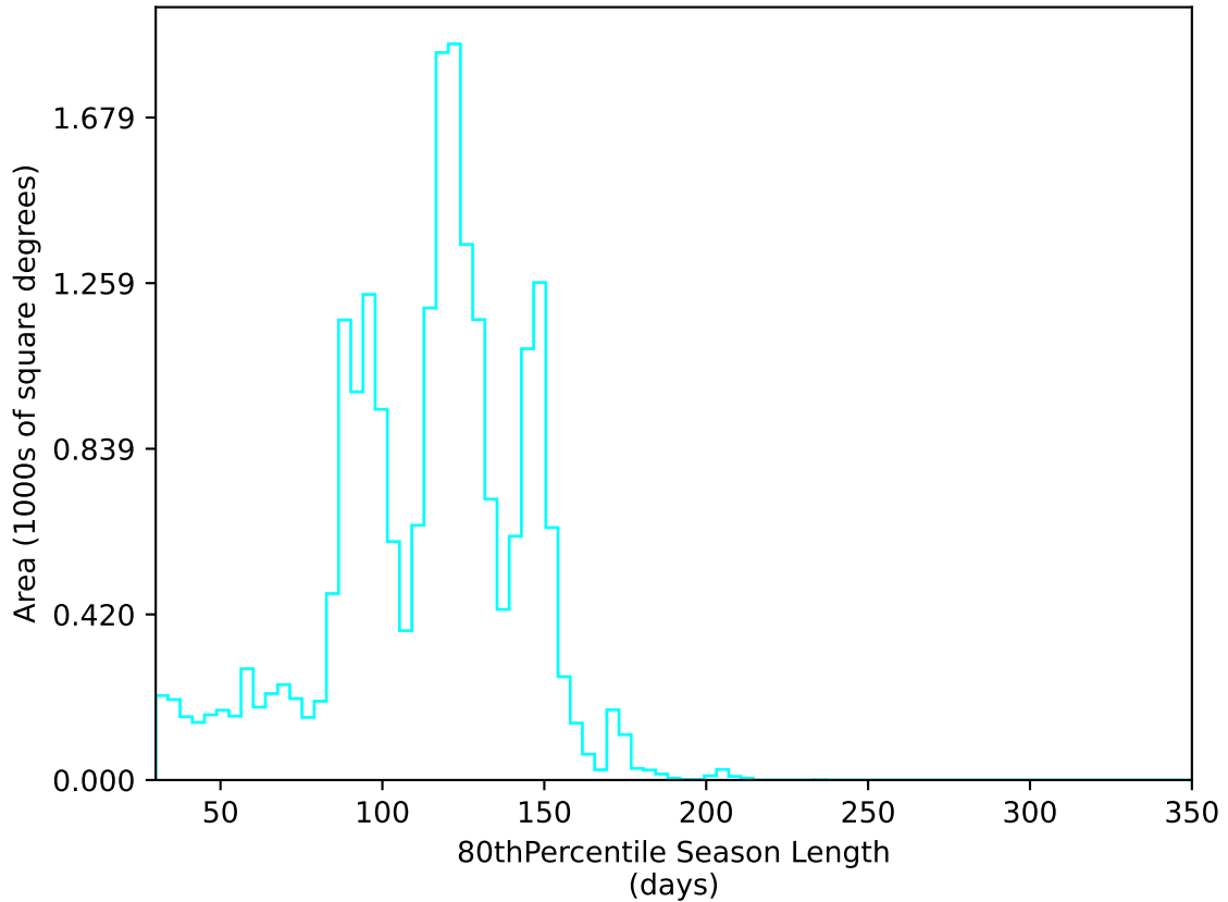
too_elab_heavy_r64_d3_ugrizy_v3.4_10yrs All sky u band: 80thPercentile Season Length
