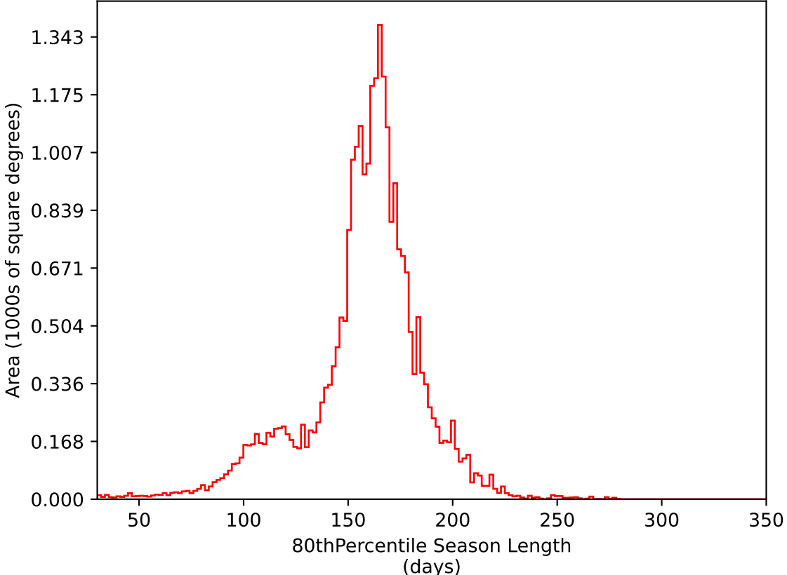
too_elab_heavy_r64_d3_ugrizy_v3.4_10yrs All sky i band: 80thPercentile Season Length
