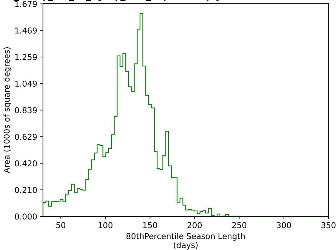
too_elab_heavy_r64_d3_ugrizy_v3.4_10yrs All sky g band: 80thPercentile Season Length
