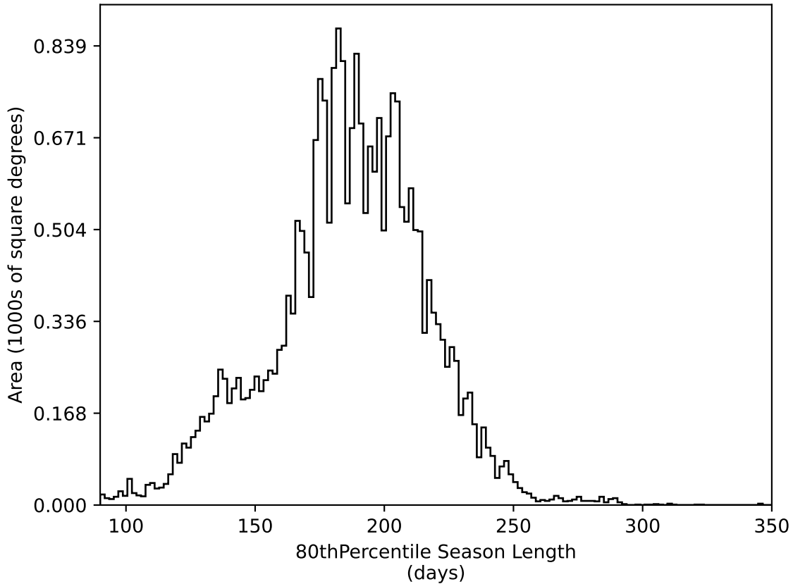
too_elab_heavy_r64_d3_ugrizy_v3.4_10yrs All sky all bands: 80thPercentile Season Length
