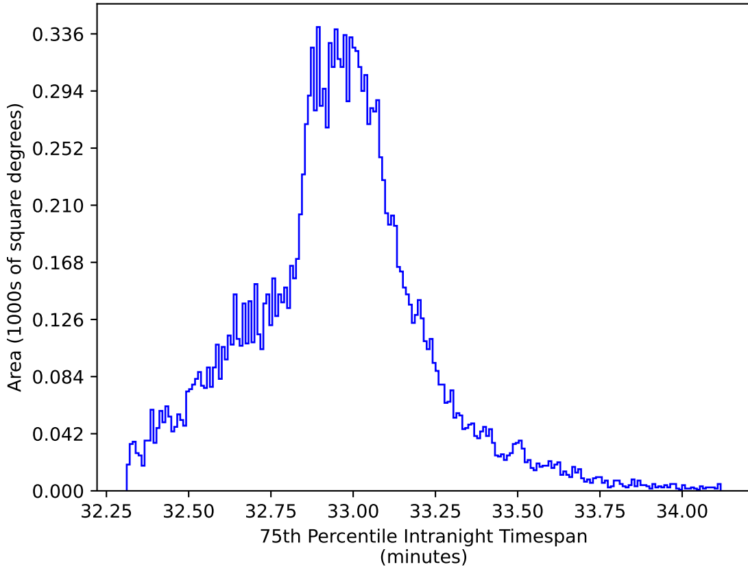
too_elab_heavy_r64_d3_ugrizy_v3.4_10yrs WFD y band: 75th Percentile Intranight Timespan
