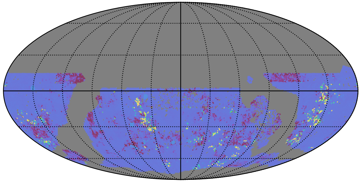
too_elab_heavy_r64_d3_ugrizy_v3.4_10yrs WFD ug bands: 75th Percentile Intranight Timespan
