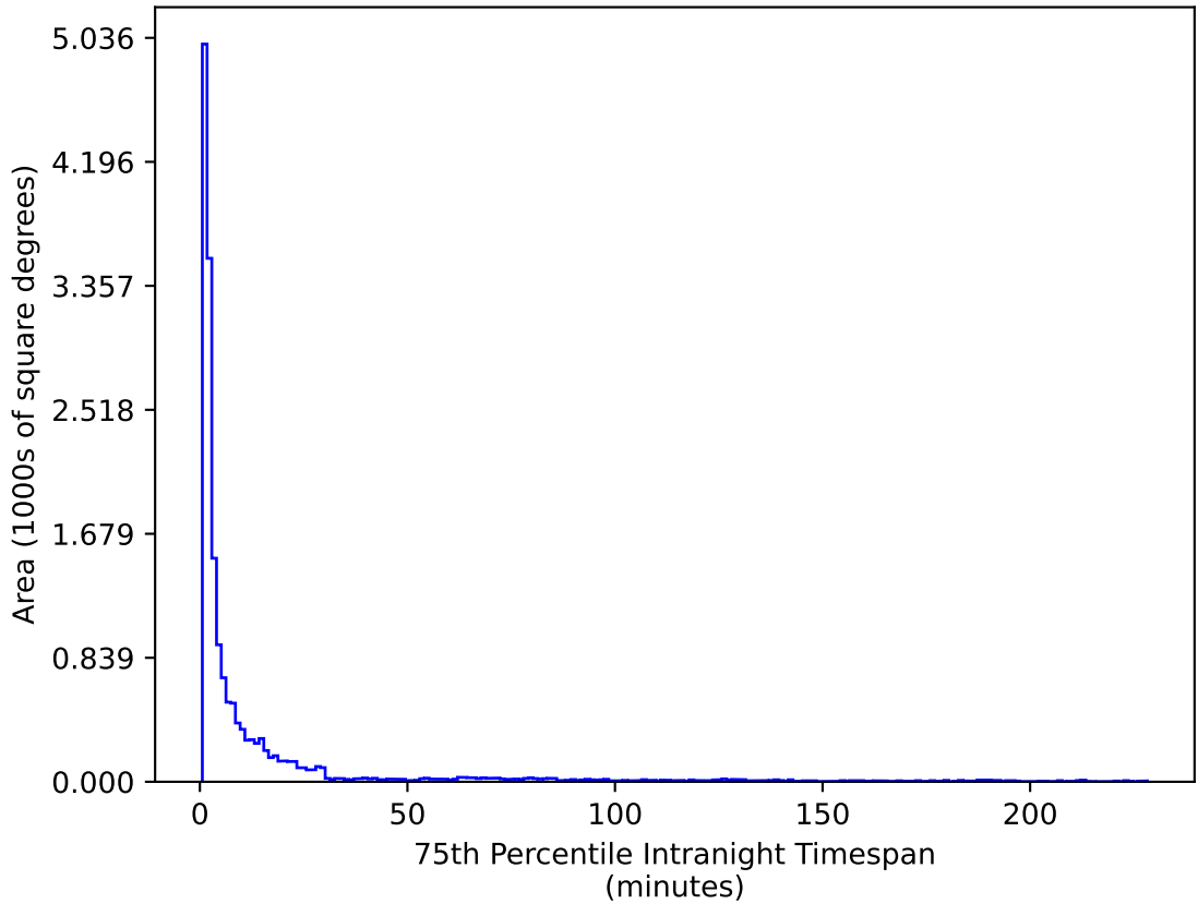
too_elab_heavy_r64_d3_ugrizy_v3.4_10yrs_WFD_u_band: 75th Percentile Intranight Timespan
