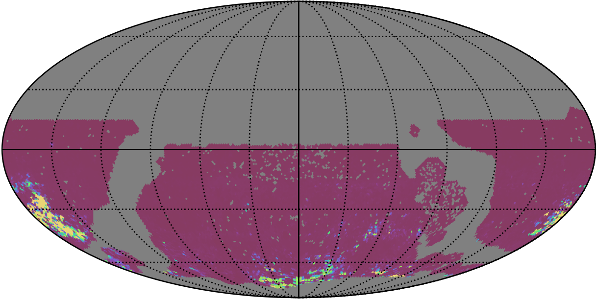
too_elab_heavy_r64_d3_ugrizy_v3.4_10yrs WFD ri bands: 75th Percentile Intranight Timespan
