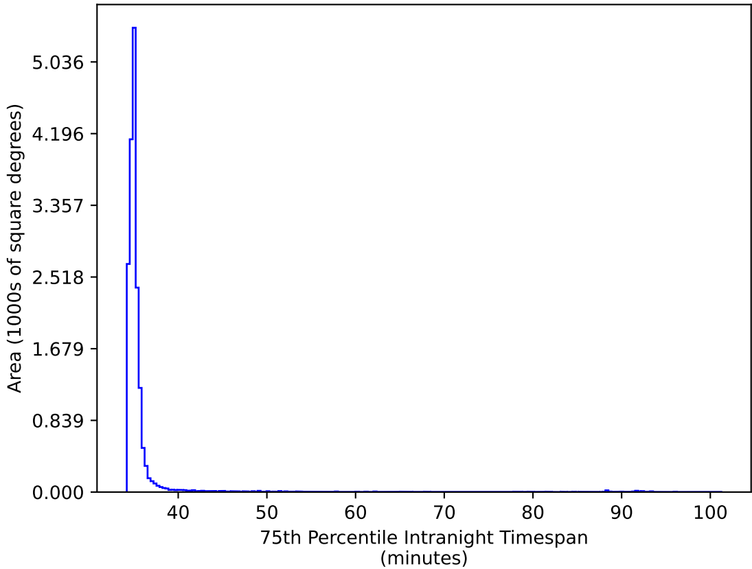
too_elab_heavy_r64_d3_ugrizy_v3.4_10yrs WFD ri bands: 75th Percentile Intranight Timespan
